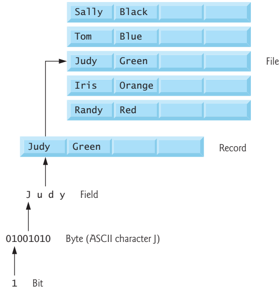
Fig. 11.1 | Data hierarchy.
