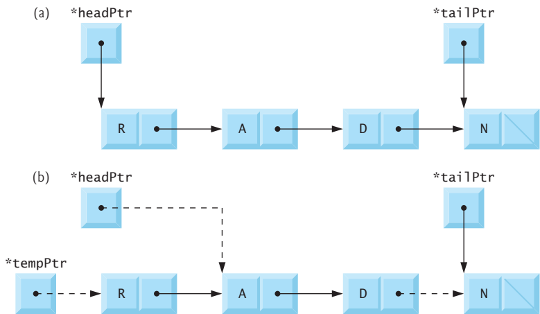
Fig. 12.16 | dequeue operation.
