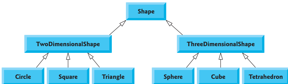
Fig. 20.3 | Inheritance hierarchy for Shapes.
